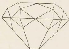
BRILLIANT.—SIDE VIEW.
